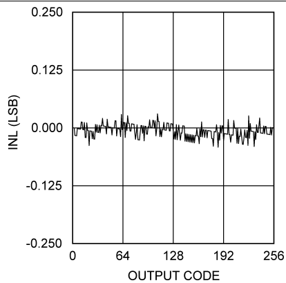
Figure 21. ADCS7478 INL
