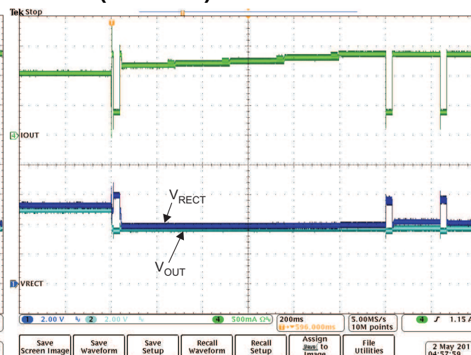
Figure 23. bq51011 Output Current Transition ( I_{LOAD} < I_{LIM} \geq I_{LIM} ) Illustrating Dynamic Communication Current Limit
