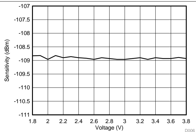
Figure 5-15. RX (50 kbps) Sensitivity vs Voltage 915 MHz
