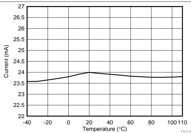
Figure 5-32. TX Current With Maximum Output Power vs Temperature, 868 MHz
