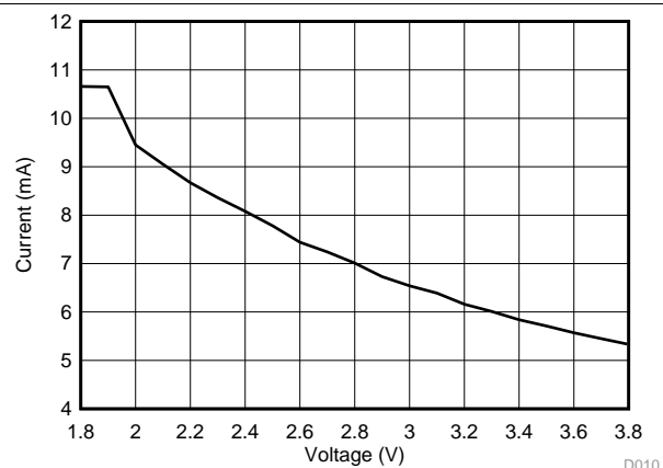
Figure 5-19. RX (50 kbps) Current vs Voltage at 915 MHz
