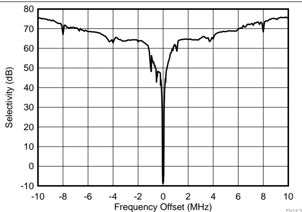
Figure 5-21. RX (50 kbps) Selectivity With Wanted Signal at 915 MHz, 3 dB Above Sensitivity Limit
