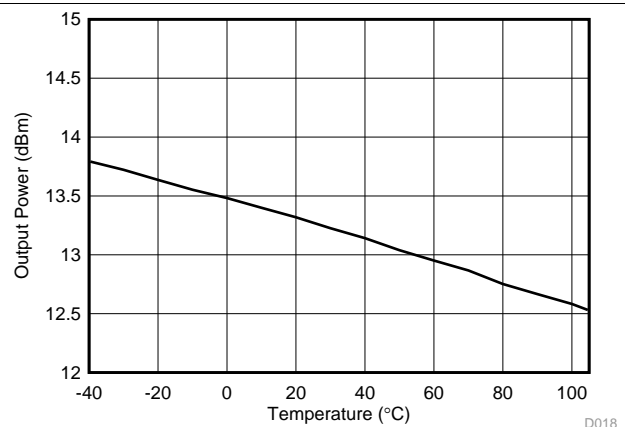
Figure 5-27. TX Maximum Output Power vs Temperature, 915 MHz
