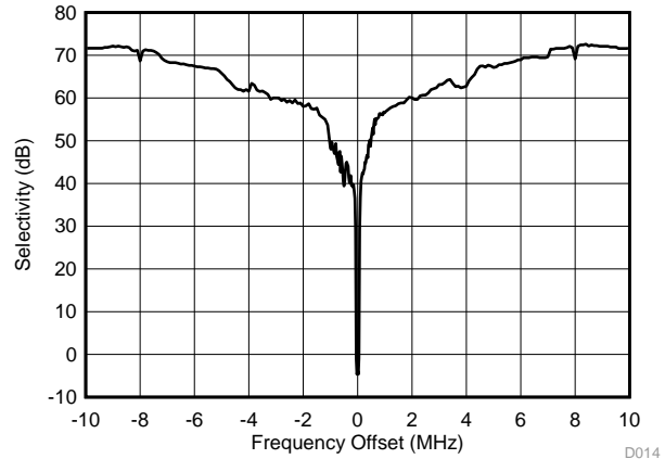
Figure 5-23. RX (50 kbps) Selectivity With Wanted Signal at 915 MHz, -96 dBm
