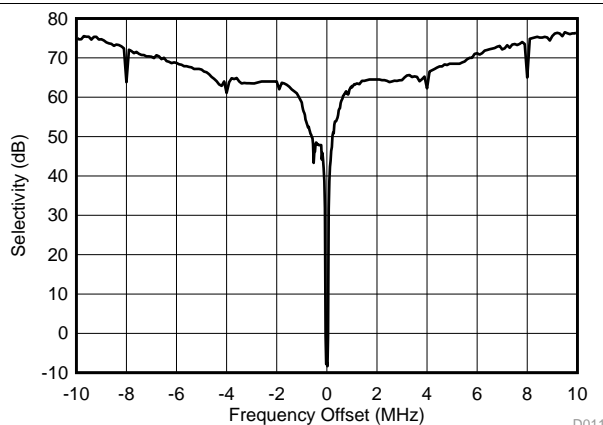
Figure 5-20. RX (50 kbps) Selectivity With Wanted Signal at 868 MHz, 3 dB Above Sensitivity Limit
