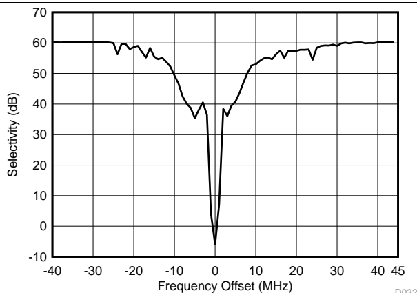
Figure 5-41. RX Bluetooth low energy Selectivity vs Frequency Offset
