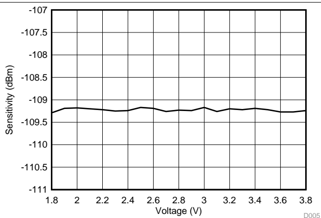
Figure 5-14. RX (50 kbps) Sensitivity vs Voltage 868 MHz
