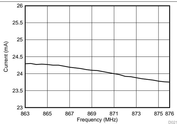
Figure 5-30. TX Current With Maximum Output Power, 863 MHz to 876 MHz
