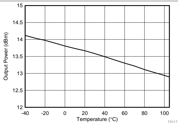
Figure 5-26. TX Maximum Output Power vs Temperature, 868 MHz
