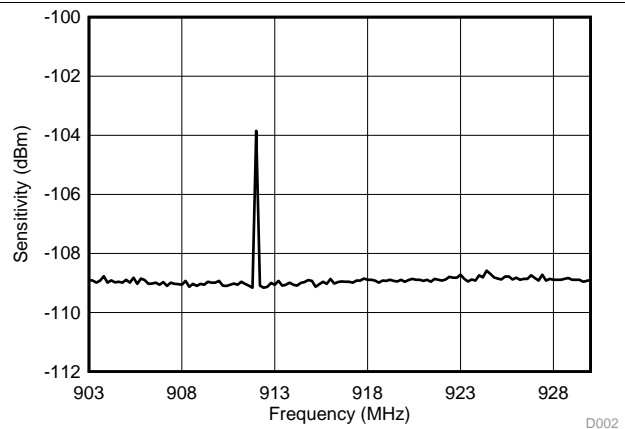
Figure 5-11. RX (50 kbps) Sensitivity vs Frequency 902 MHz to 928 MHz
