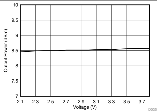
Figure 5-44. TX Bluetooth low energy Maximum Output Power vs VDD5, 2440 MHz
