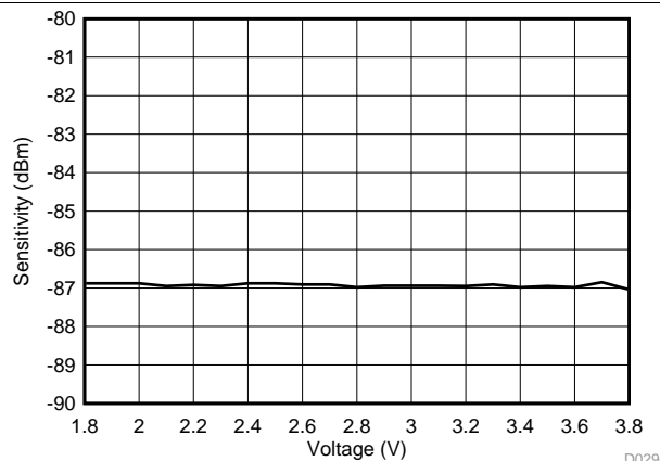
Figure 5-38. RX Bluetooth low energy Sensitivity vs Voltage, 2440 MHz
