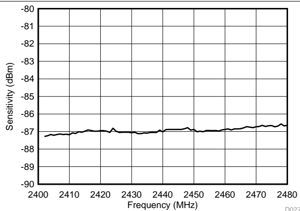
Figure 5-36. RX Bluetooth low energy Sensitivity vs Frequency 2402 MHz to 2480 MHz
