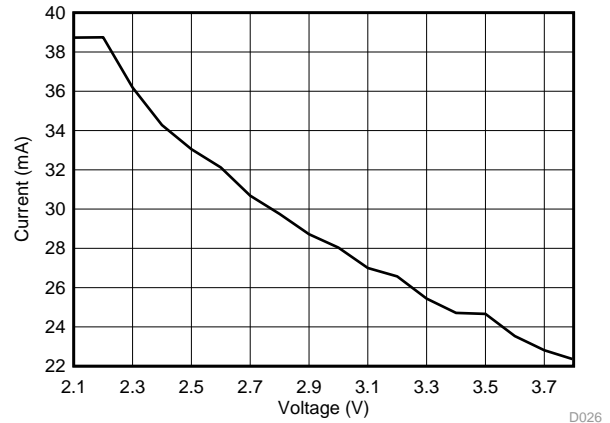
Figure 5-35. TX Current With Maximum Output Power vs Voltage, 915 MHz
