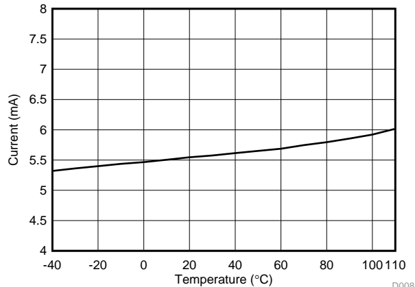
Figure 5-17. RX (50 kbps) Current vs Temperature at 915 MHz
