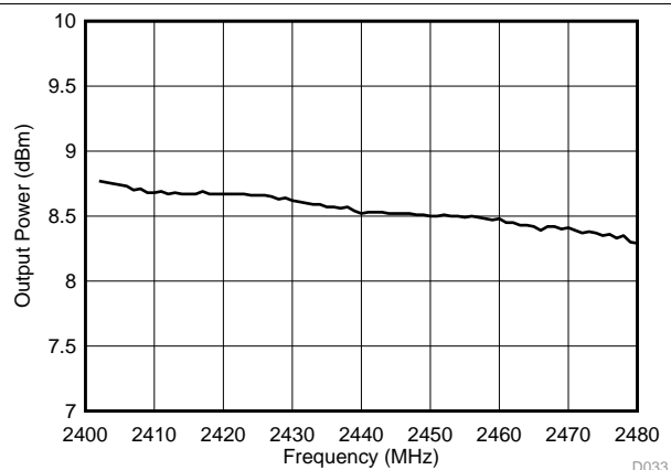
Figure 5-42. TX Bluetooth low energy Maximum Output Power, 2402 MHz to 2480 MHz
