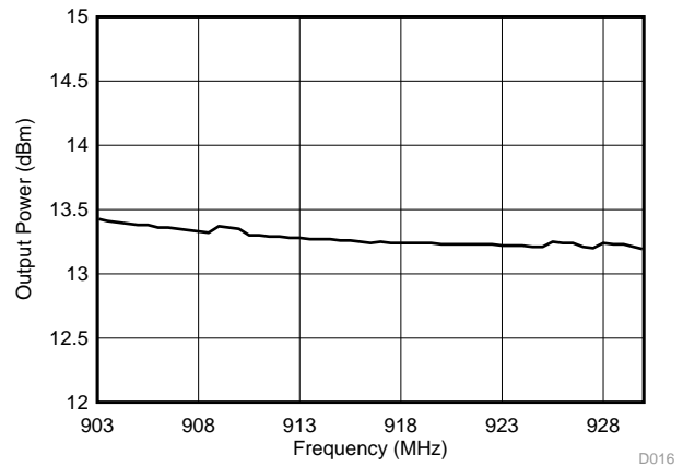
Figure 5-25. TX Maximum Output Power, 902 MHz to 928 MHz
