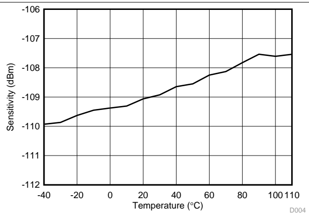
Figure 5-13. RX (50 kbps) Sensitivity vs Temperature 915 MHz
