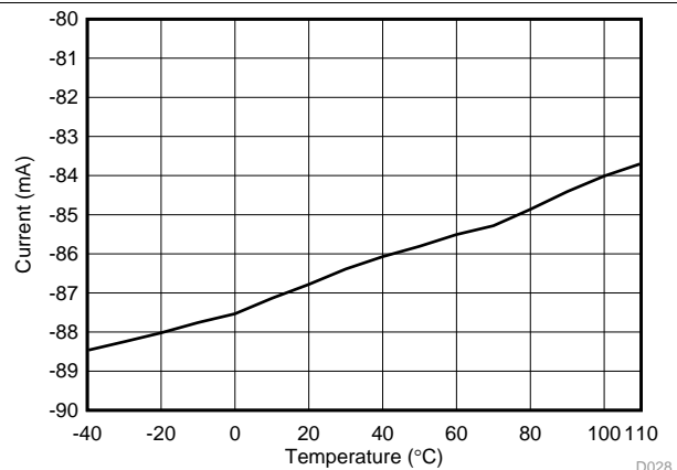
Figure 5-37. RX Bluetooth low energy Sensitivity vs Temperature 2440 MHz
