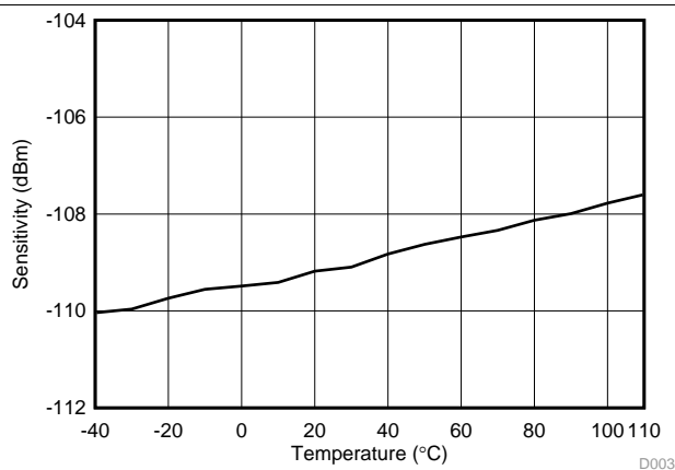
Figure 5-12. RX (50 kbps) Sensitivity vs Temperature 868 MHz
