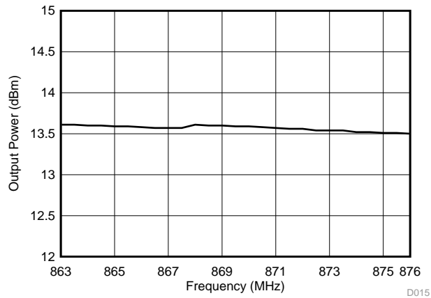
Figure 5-24. TX Maximum Output Power, 863 MHz to 876 MHz
