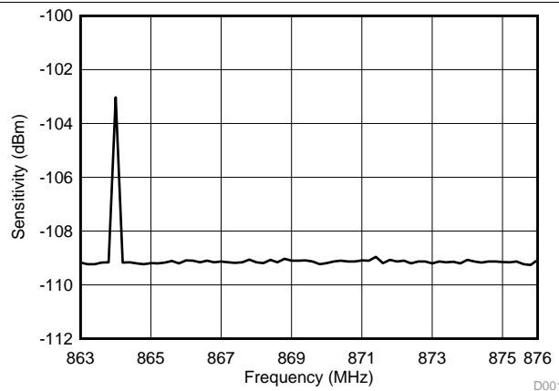
Figure 5-10. RX (50 kbps) Sensitivity vs Frequency 863 MHz to 876 MHz
