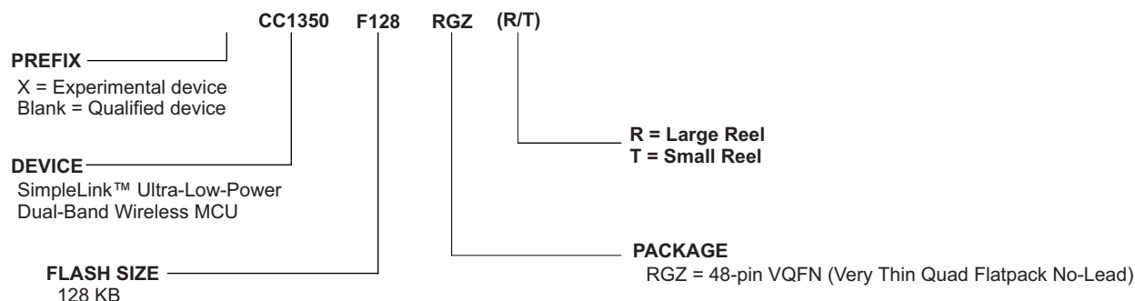
Figure 8-1. Device Nomenclature
