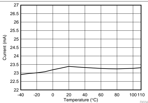
Figure 5-33. TX Current With Maximum Output Power vs Temperature, 915 MHz
