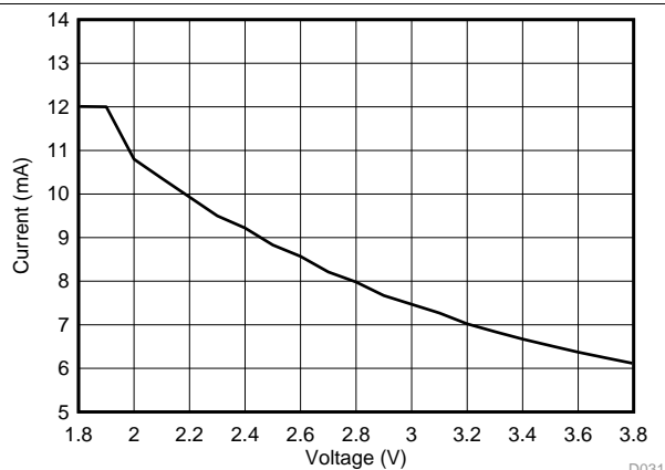
Figure 5-40. RX Bluetooth low energy Current vs Voltage at 2440 MHz
