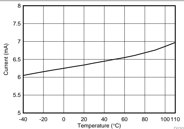
Figure 5-39. RX Bluetooth low energy Current vs Temperature at 2440 MHz
