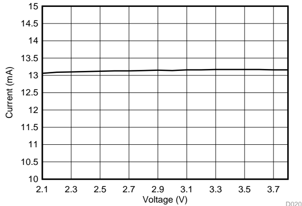
Figure 5-29. TX Maximum Output Power vs VDDSD, 915 MHz
