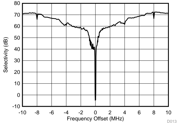
Figure 5-22. RX (50 kbps) Selectivity With Wanted Signal at 868 MHz, -96 dBm
