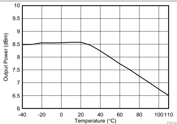
Figure 5-43. TX Bluetooth low energy Maximum Output Power vs Temperature, 2440 MHz
