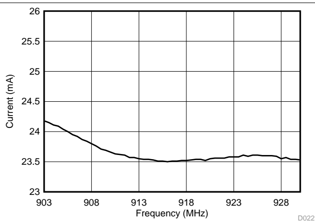
Figure 5-31. TX Current With Maximum Output Power, 902 MHz to 928 MHz
