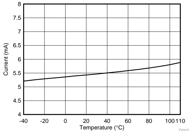
Figure 5-16. RX (50 kbps) Current vs Temperature at 868 MHz
