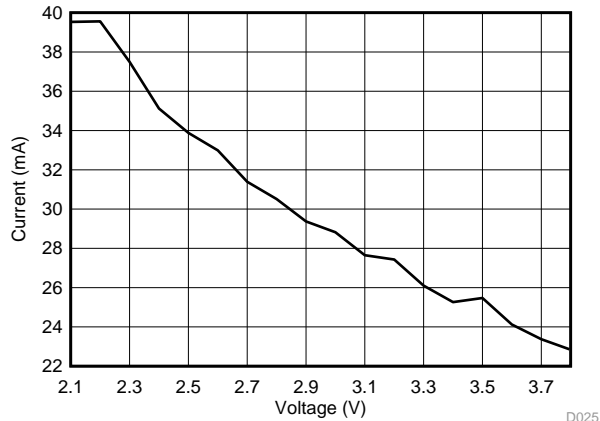
Figure 5-34. TX Current With Maximum Output Power vs Voltage, 868 MHz
