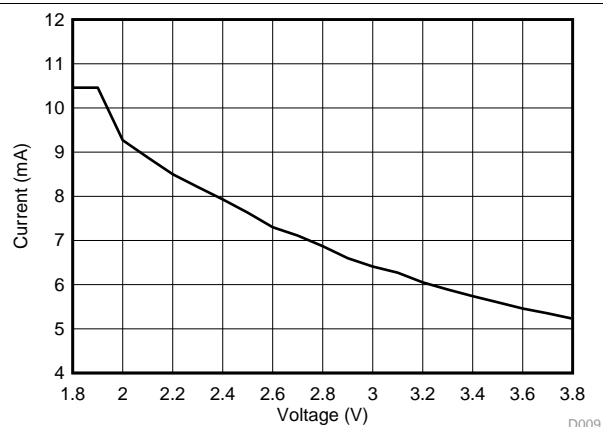
Figure 5-18. RX (50 kbps) Current vs Voltage at 868 MHz
