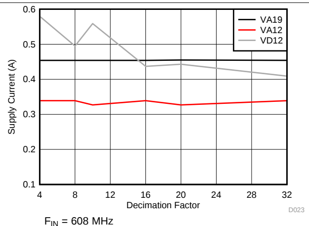
Figure 14. Supply Current vs Decimation Setting
