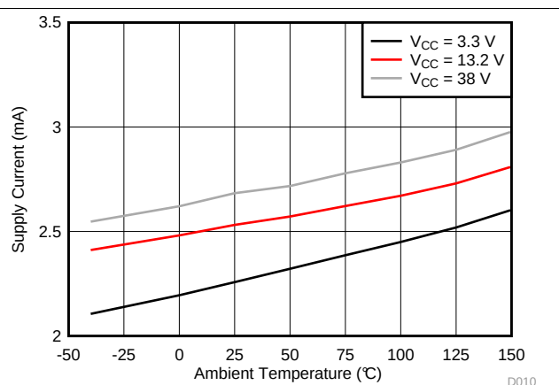
Figure 2. I CC vs Temperature
