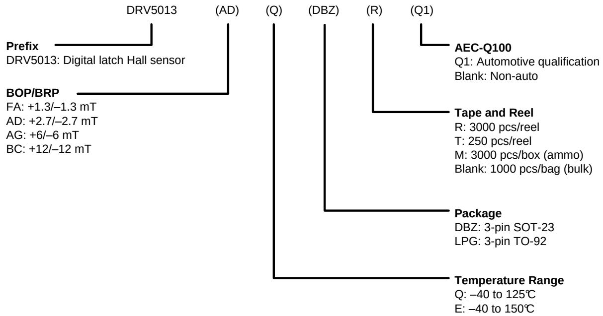
Figure 24. Device Nomenclature
