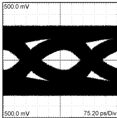
Figure 23. A 2.5 Gbps NRZ PRBS-23 without PE After 30\"
