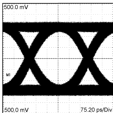
Figure 25. A 2.5 Gbps NRZ PRBS-23 with High PE After 30\"
