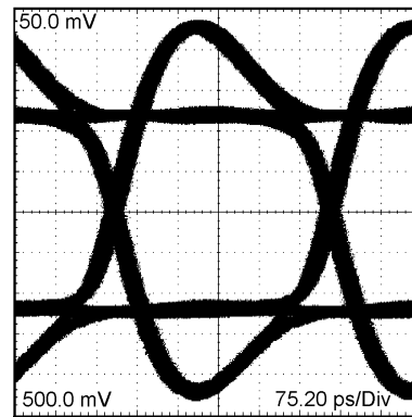
Figure 24. A 2.5 Gbps NRZ PRBS-23 with High PE After 2\"
