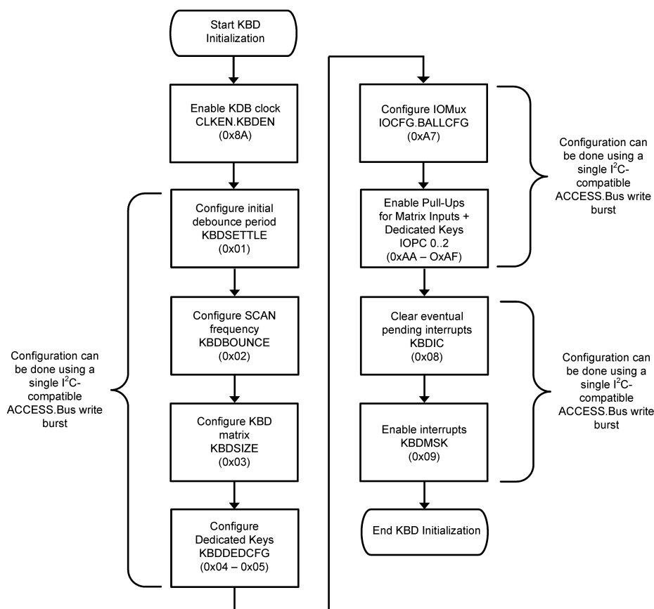
Figure 6. Keyscan Initialization
