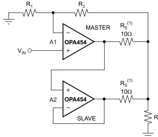
Figure 65. Parallel Amplifiers Increase Output Current Capability
