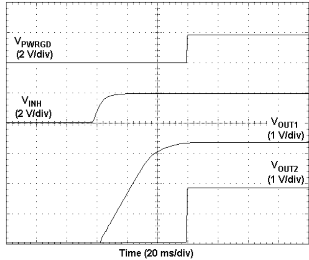
Figure 37. Sequencing Waveforms
