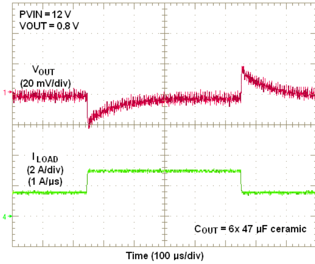
Figure 16. P_{VIN} = 12V , V_{OUT} = 0.8V , 1.5A Load Step
