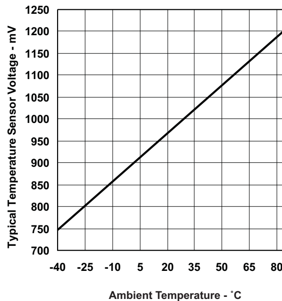
Figure 5-16. Typical Temperature Sensor Voltage
