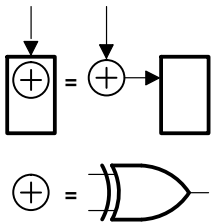
Figure 10. 18-Bit PSA/PRPG Configuration ( 1\overline{OEAB} = 2\overline{OEAB} = 1 , 1\overline{OEBA} = 2\overline{OEBA} = 0 )
