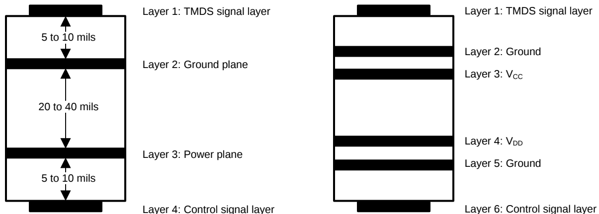
Figure 32. Recommended 4- or 6-Layer Stack for a Receiver PCB Design
