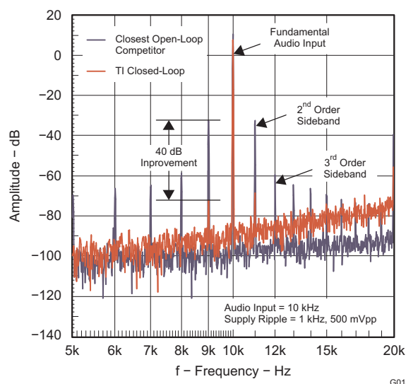
Figure 1. Supply Ripple Intermod Distortion
