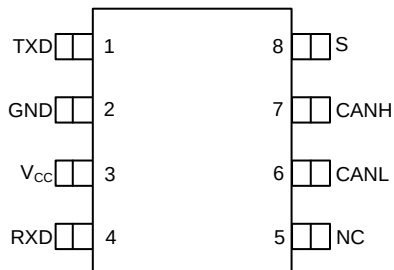
D Package for Base, (H), (G), and (HG) Devices 8 PIN (SOIC) Top View
