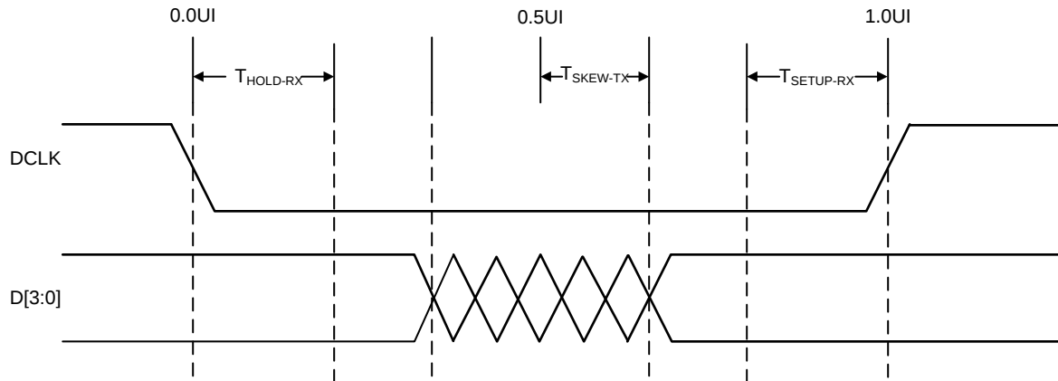
Figure 2. DPHY HS RX and TX Timing
