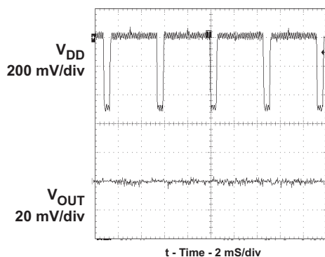
GSM POWER SUPPLY REJECTION VS TIME
