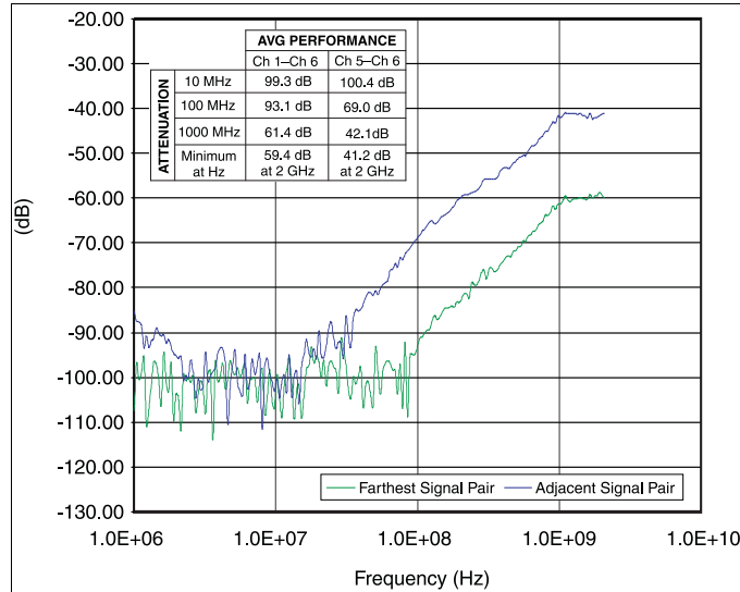
Figure 1. Channel-to-Channel Crosstalk
