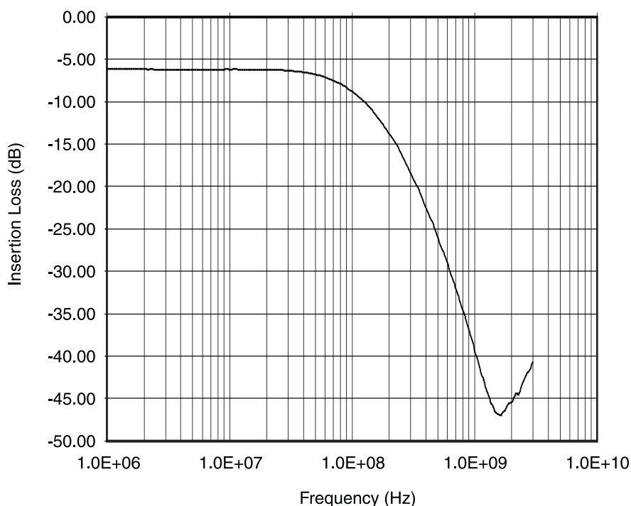
Figure 8. Frequency Response Data (0-V Bias)
