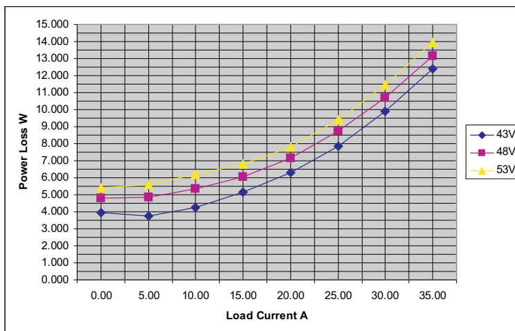
Figure 56. . Power Dissipation
