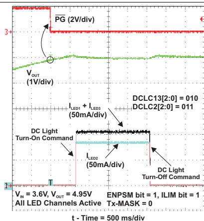
Figure 80. DC-Light Operation (HC_SEL = 1)
