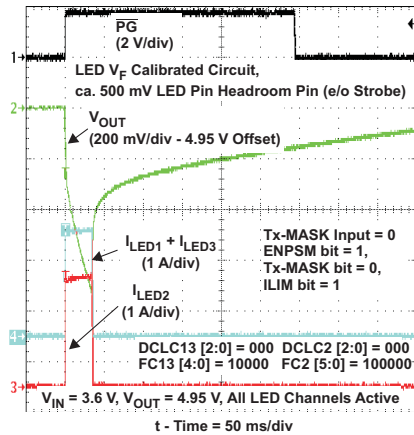
Figure 84. Flash Sequence (HC_SEL = 1)
