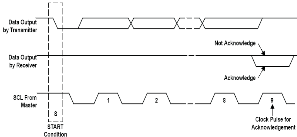
Figure 42. Acknowledge on the I²C Bus
