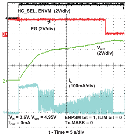
Figure 78. Storage Capacitor Charge-Up (HC_SEL = 1)
