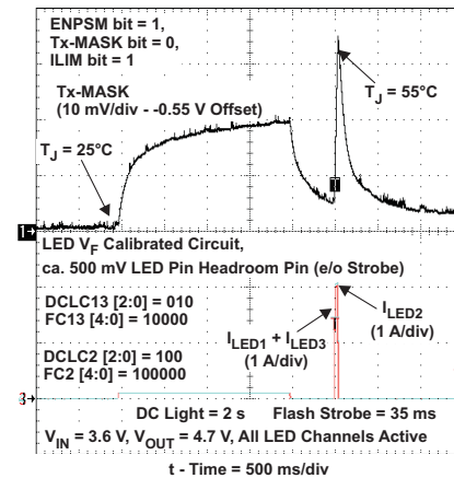
Figure 85. Junction Temperature Monitoring (HC_SEL = 1)
