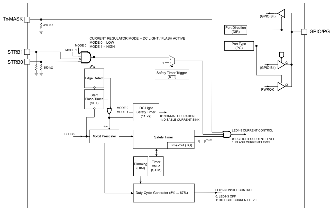
Figure 30. Timer Block Diagram
