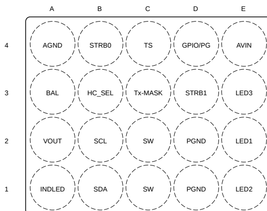
Pin Functions
