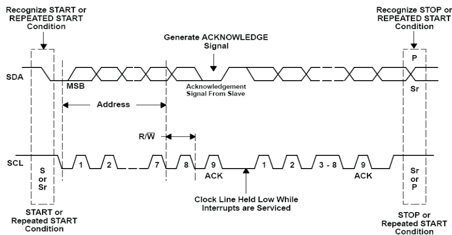
Figure 43. Bus Protocol
