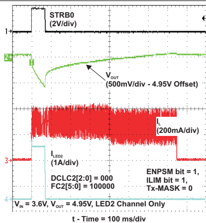
Figure 82. Flash Sequence (HC_SEL = 1)
