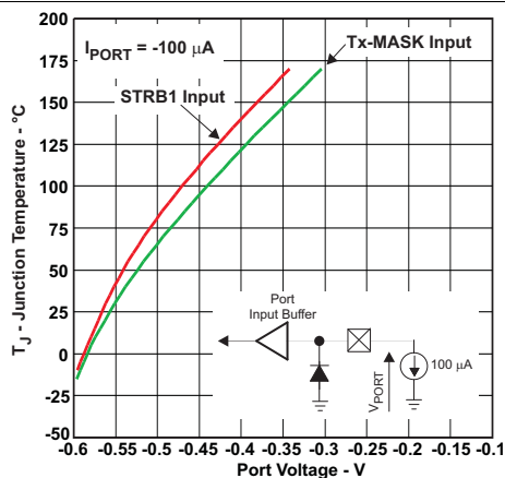
Figure 64. Junction Temperature vs Port Voltage
