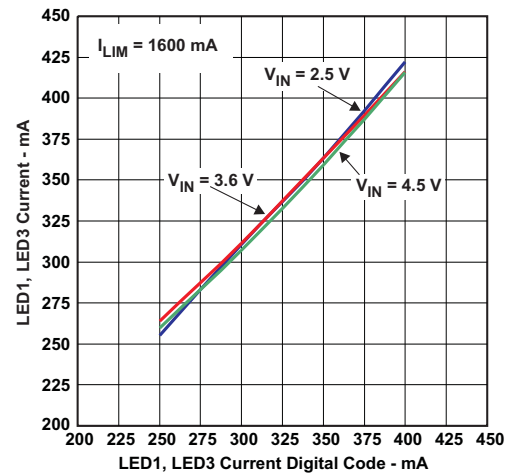
Figure 12. LED1 and LED3 Current vs LED1 and LED3 Current Digital Code (HC_SEL = 0)
