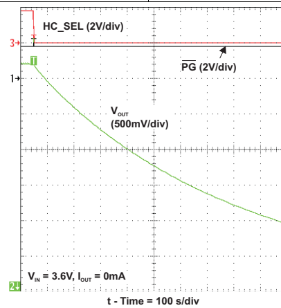
Figure 86. Shutdown (HC_SEL = 1)
