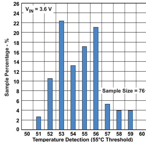
Figure 26. Temperature Detection Threshold
