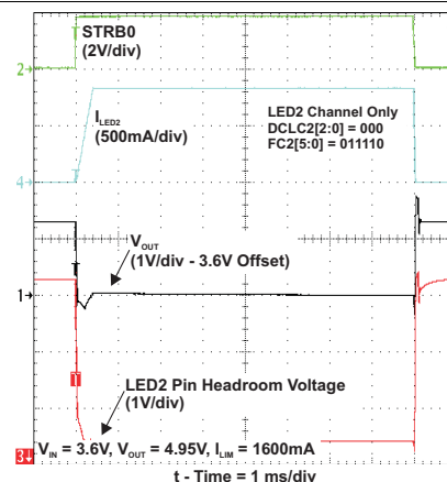
Figure 65. Flash Sequence (HC_SEL = 0)
