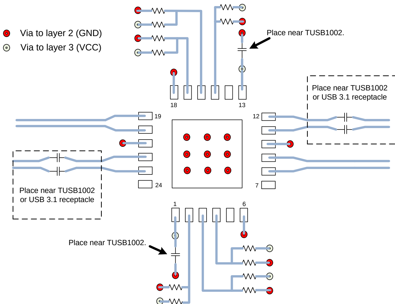
Figure 20. Example Layout
