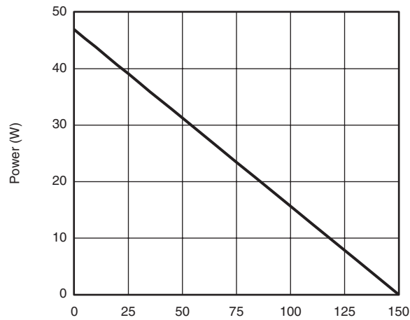
Power Junction-to-Case
