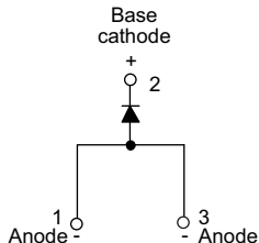
VS-40APS16PbF VS-40APS16-M3
