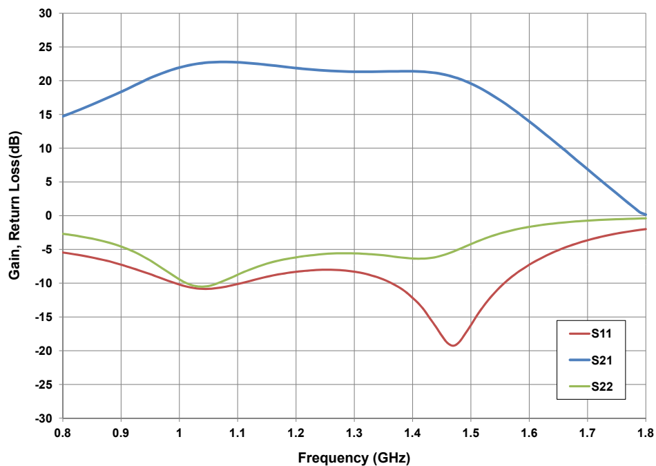
Figure 2. - Typical Large Signal Response of CGHV40030-AMP Application Circuit
