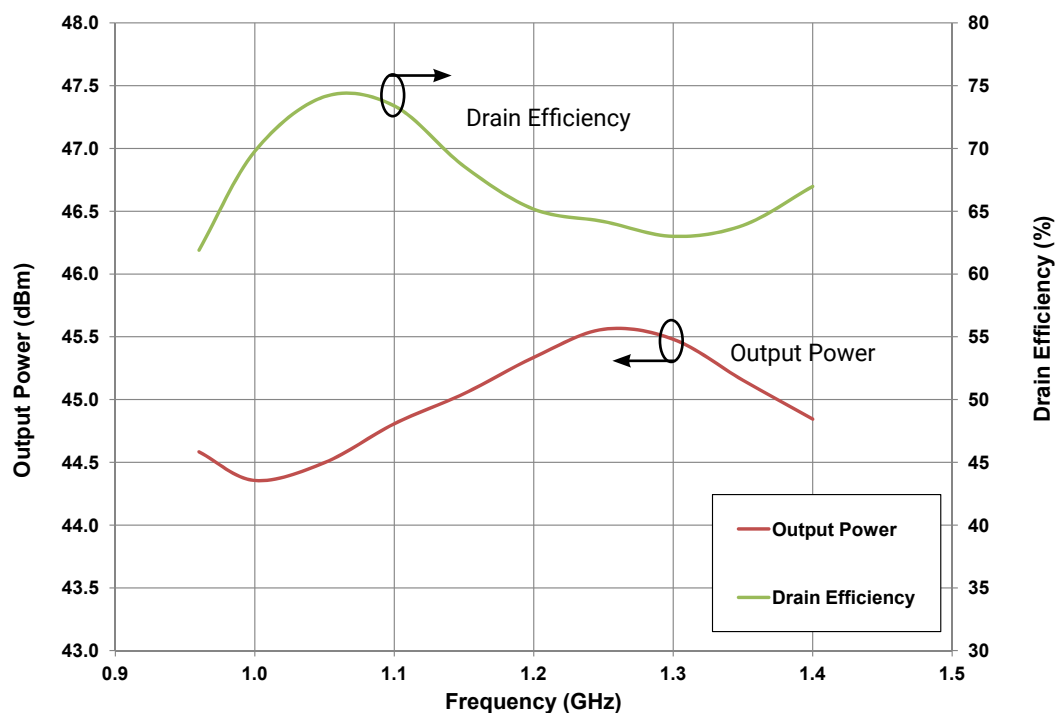
Figure 2. - Typical Large Signal Response of CGHV40030-AMP Application Circuit
