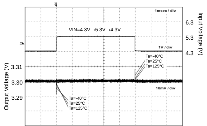
Figure 28. VIN Response
