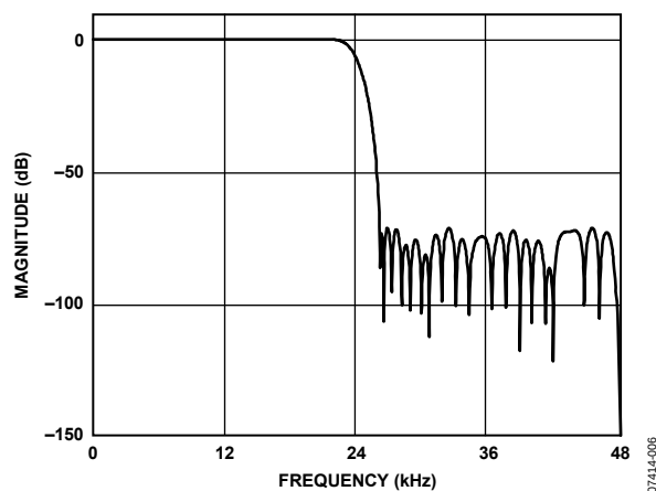
Figure 8. DAC Stop-Band Filter Response, 48 kHz
