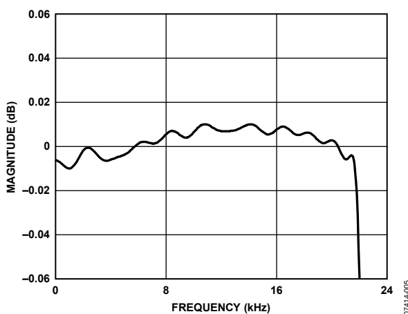
Figure 7. DAC Pass-Band Filter Response, 48 kHz
