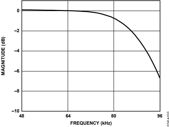
Figure 12. DAC Stop-Band Filter Response, 192 kHz
