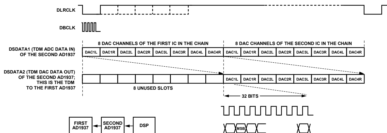
Figure 22. Single-Line Daisy-Chain TDM Mode 16-Channel 48 kHz DAC Configuration
