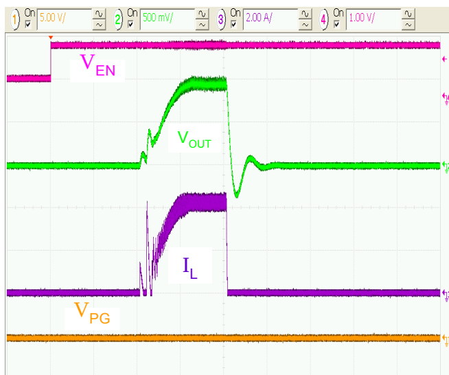
Figure 25. Over-Current at Startup, R_{LOAD}=200\text{ m}\Omega , 50 μs/div.
