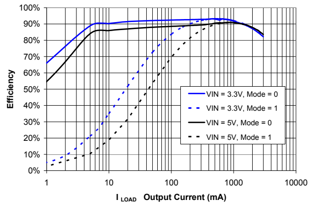
Figure 4. Efficiency vs. I_{LOAD} at V_{OUT}=1.8\text{ V}
