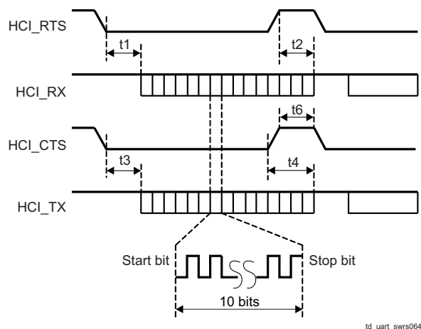
Figure 4-2. UART Timing
