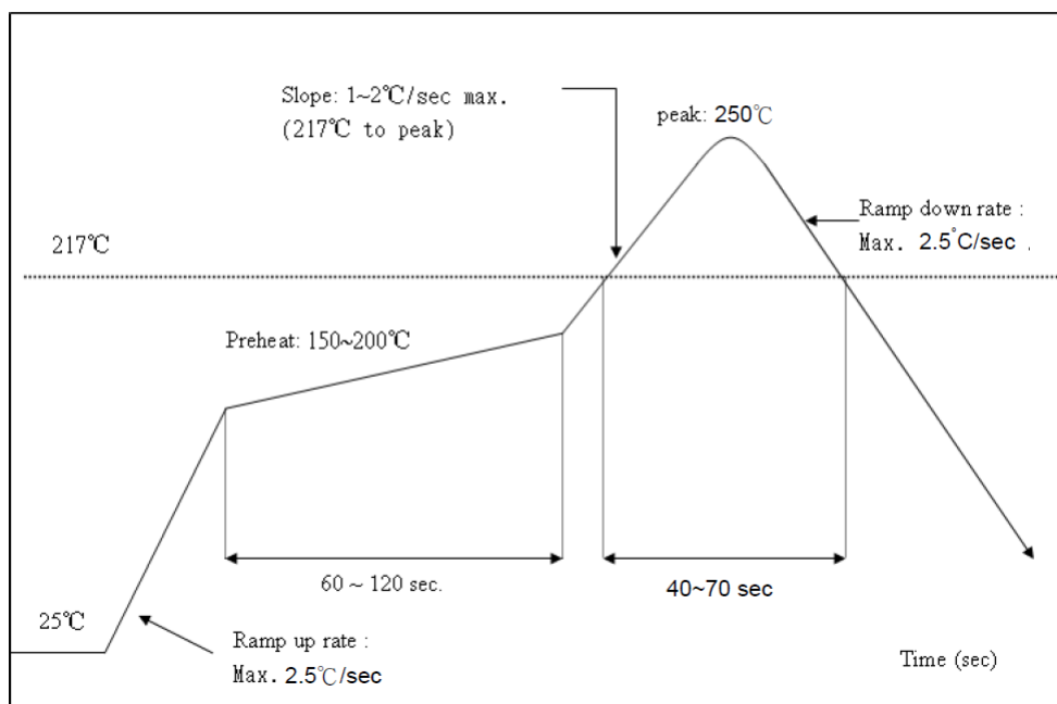
Figure 6-16. Reflow Profile
