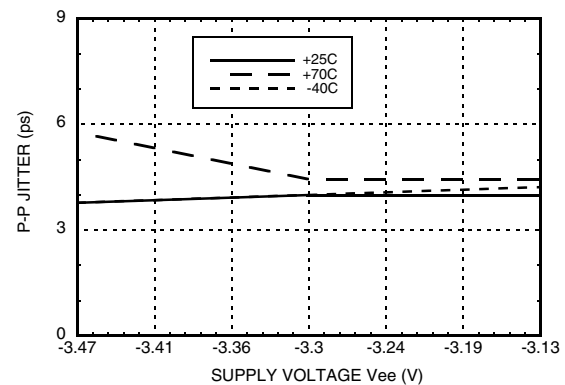
Peak-to-Peak Jitter vs. Supply Voltage [1][2][3][4]
