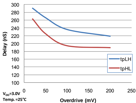
Figure 11. Propagation Delay vs. Input Overdrive
