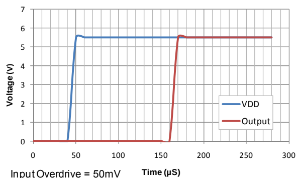
Figure 13. Power-Up Delay
