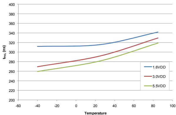
Figure 9. Propagation Delay ( t_{PLH} ) vs. Temperature
