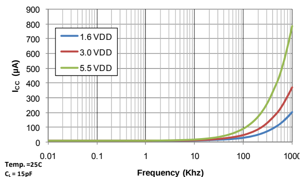
Figure 5. Supply Current vs. Output Transition Frequency
