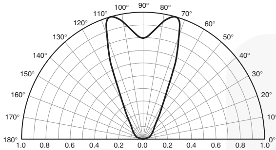
Figure 7. Radiation Diagram
