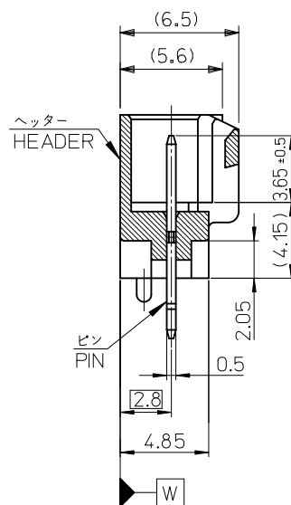
SECT. X-X
