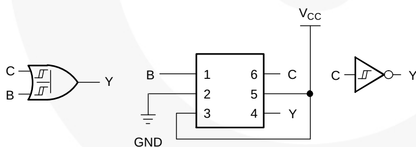
Figure 6. 2-Input OR Gate
