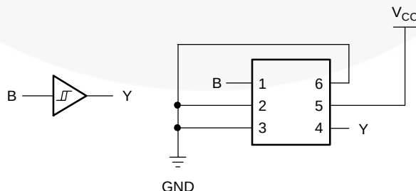
Figure 8. Buffer
