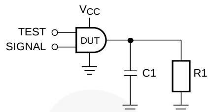
Figure 4. Test Circuit
