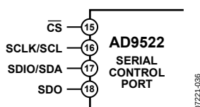
Figure 63. Serial Control Port
