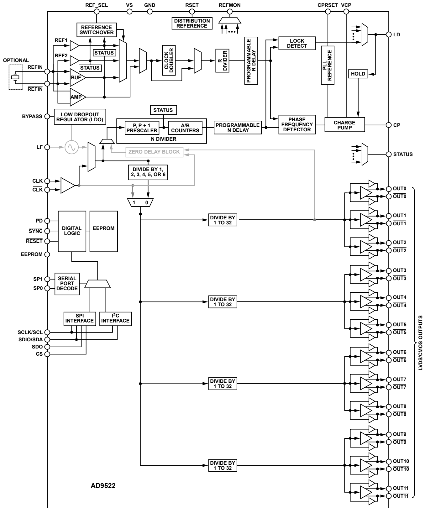
Figure 38. High Frequency Clock Distribution—CLK or External VCO &gt; 1600 MHz (Mode 2)
