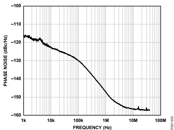
Figure 30. Phase Noise (Absolute) Clock Generation; Internal VCO at 212.2 MHz; PFD = 15.36 MHz; LBW = 40 kHz; LVDS Output = 122.88 MHz
