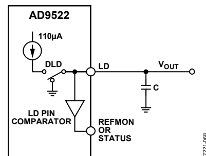
Figure 46. Current Source Digital Lock Detect
