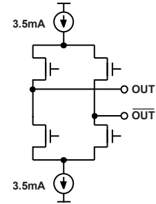
Figure 53. LVDS Output Simplified Equivalent Circuit with 3.5 mA Typical Current Source
