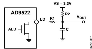
Figure 45. Example of Analog Lock Detect Filter Using N-Channel Open-Drain Driver
