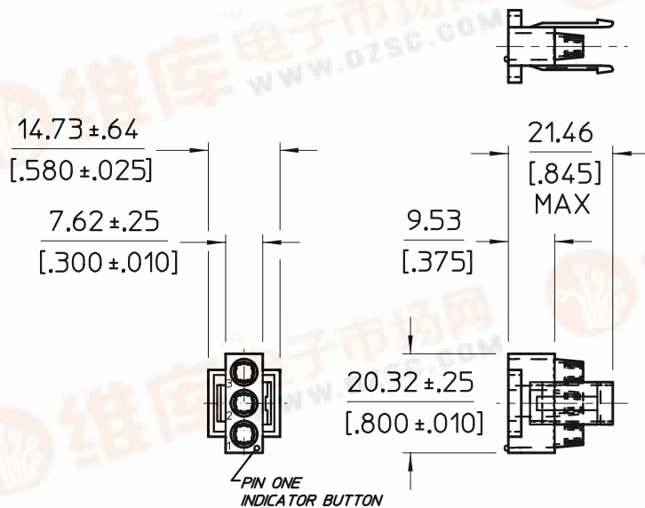
CONN HOUSING PLUG- REAR
