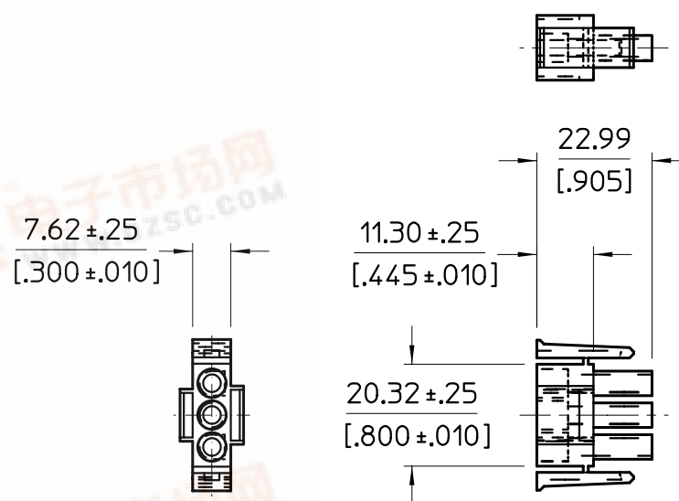
CONN HOUSING PLUG- FRONT
