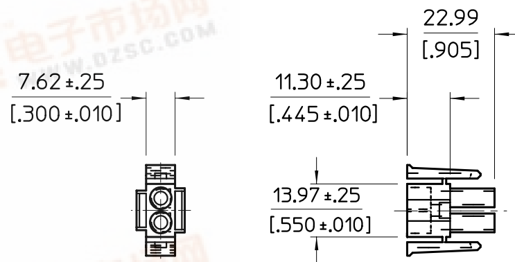
CONN HOUSING PLUG- FRONT
