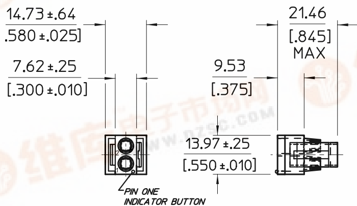
CONN HOUSING PLUG- REAR
