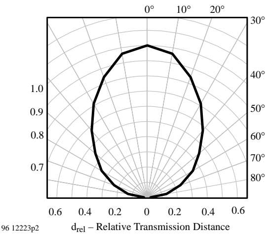
Figure 13. Directivity
