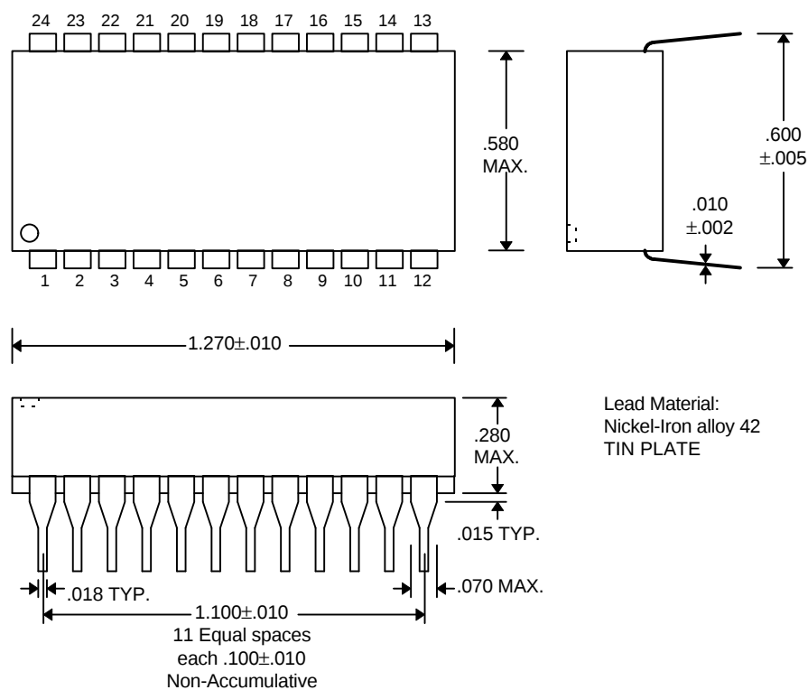
DIP (2214-xxz)
