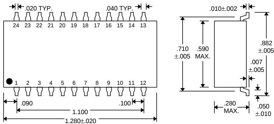
Gull-Wing (2214-xxzC4)
