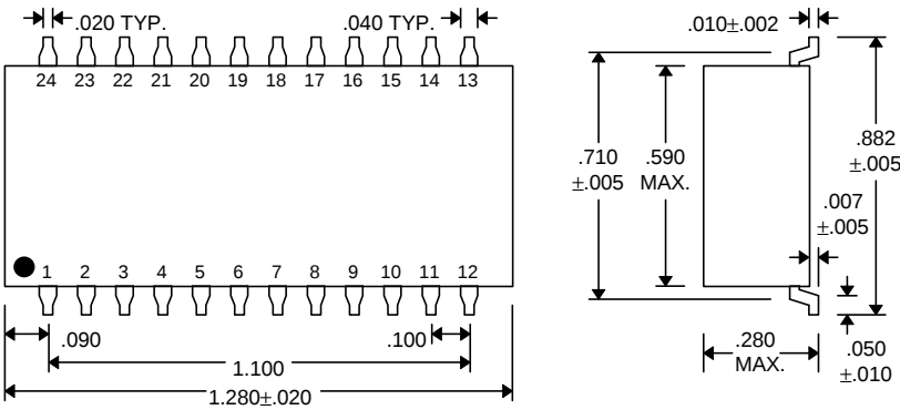
Gull-Wing (2214-xxzC4)
