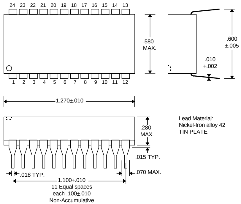
DIP (2214-xxz)
