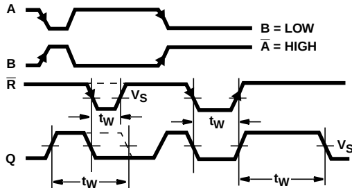
FIGURE 1. OUTPUT PULSE CONTROL USING RESET INPUT ( \bar{R} ) PULSE FOR 123
