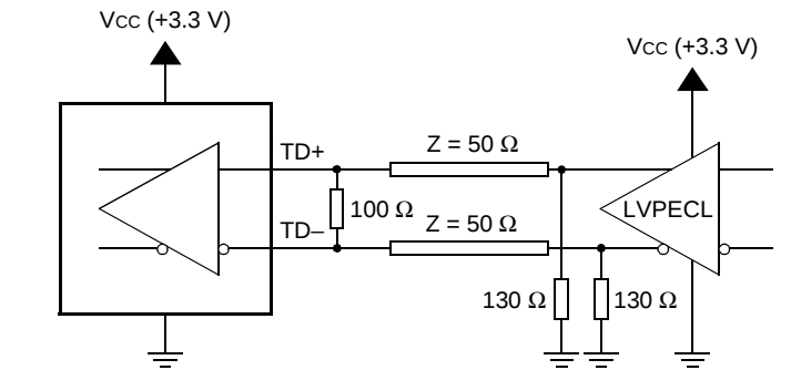
A. Transmitter Interface (LVPECL to LVPECL)
