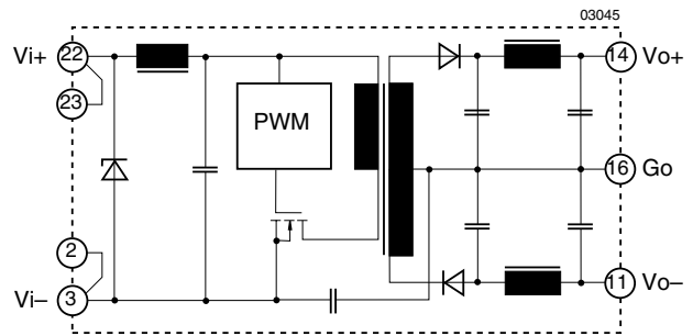
Fig. 2 Block diagram for dual output types. Standard industrial pinout.
