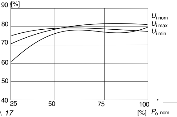
Fig. 17 Efficiency versus input voltage and load. Typical values (48IMS6 -1212-9)
