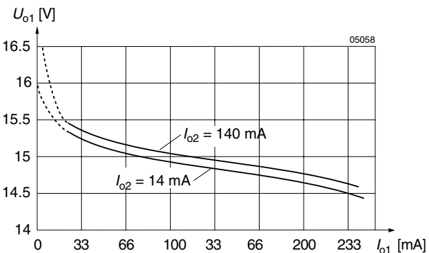
Fig. 14 Cross load regulation of dual output units. U_{o1} versus I_{o1} (typ) for various I_{o2} (48IMS6-1515-9).
