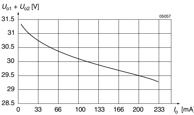
Fig. 13 U_o versus I_o (typ) of dual output units ( 15 V), with 30 V load connected to Vo+ and Vo-.
