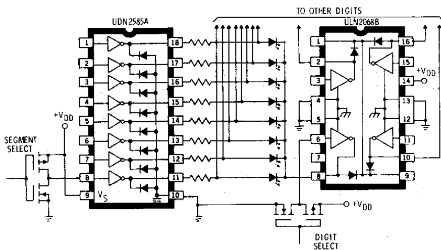
COMMON-CATHODE LED DRIVER
