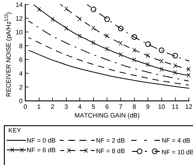
Figure 1. Receiver Noise
