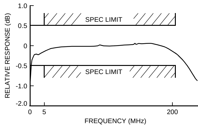
Figure 2. Frequency Response
