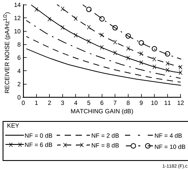
Figure 1. Receiver Noise
