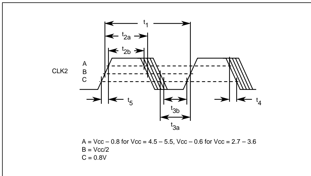
Figure 11. CLK2 Waveform
