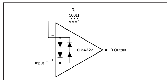
FIGURE 2. Pulsed Operation.
