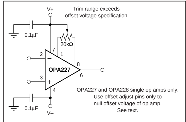
FIGURE 1. OPA227 Offset Voltage Trim Circuit.
