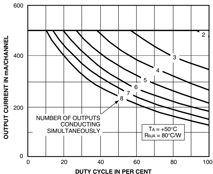
ALLOWABLE COLLECTOR CURRENT AS A FUNCTION OF DUTY CYCLE
