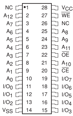
SOIC Package (J, W) (K, X)
