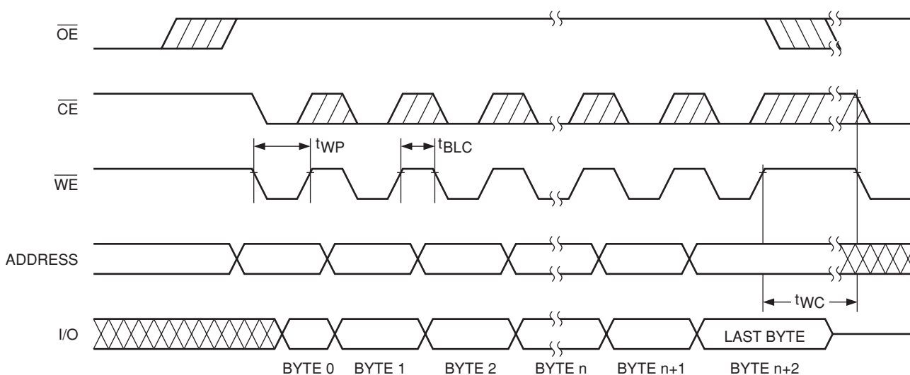
Figure 6. Page Mode Write Cycle
