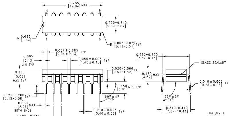
Order Number CD4029BMJ or CD4029BCJ NS Package Number J16A
